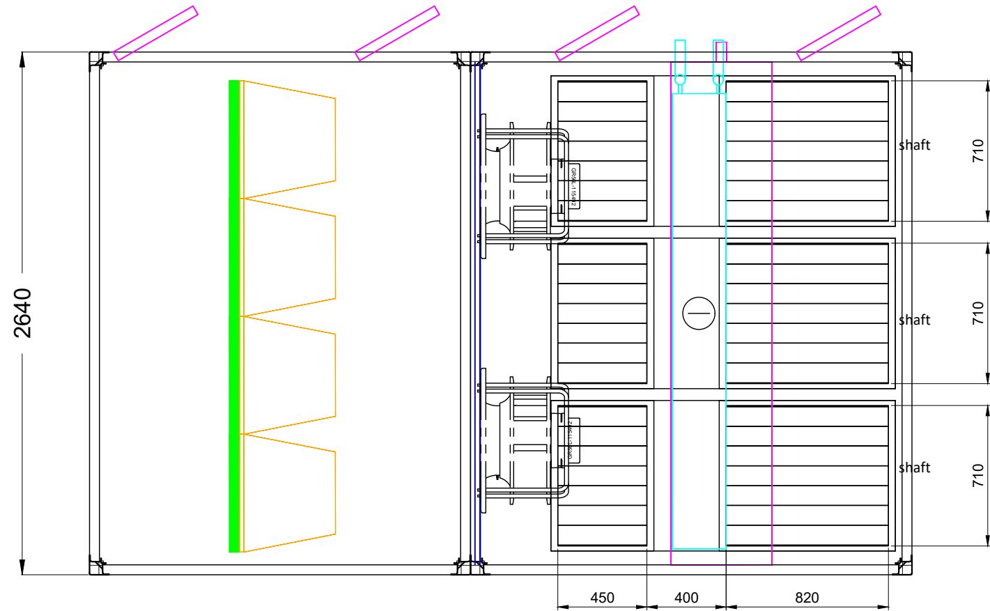
Top View
